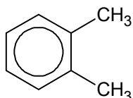
o-xylen
