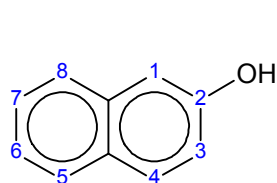
2-naftol
