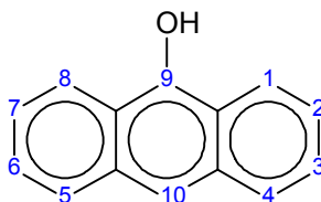
9-anthrol
